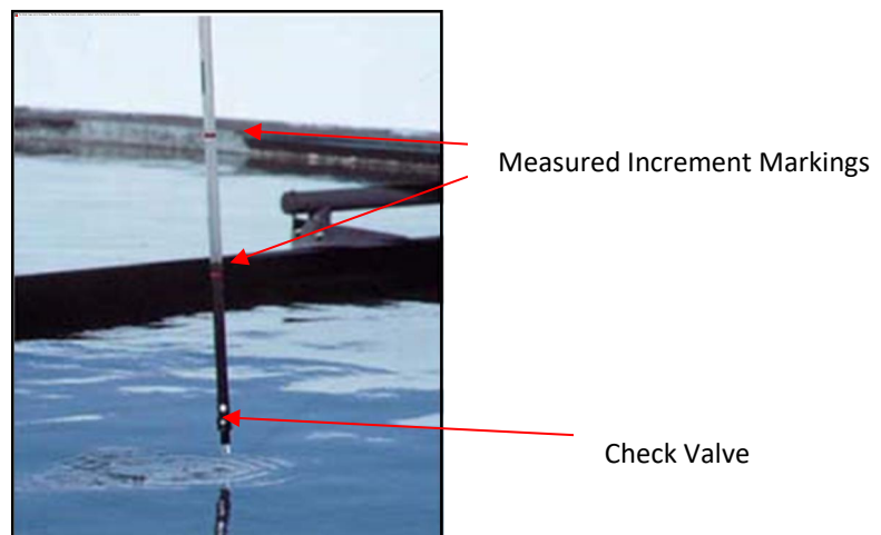
Figure 3: Photo of Sludge Judge®
