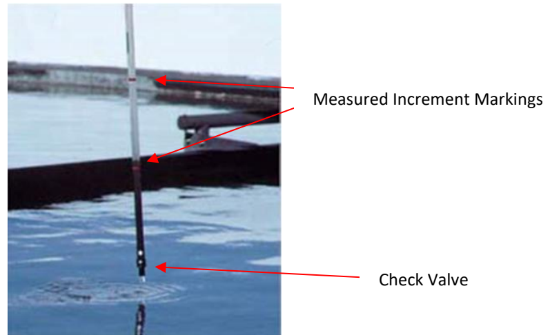
Figure 3: Photo of Sludge Judge® Source: GENEQ Inc.(n.d)
